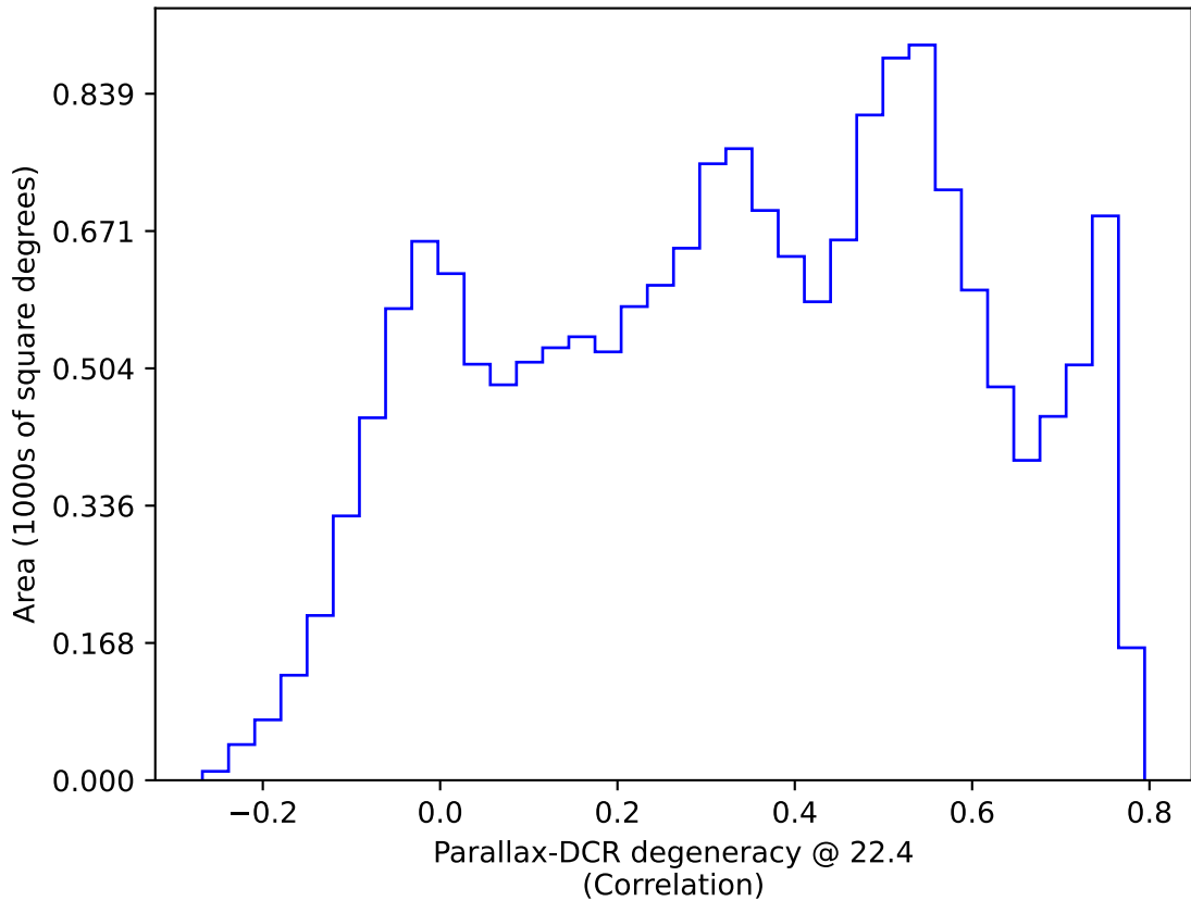
too_ignore_100_1v3.4_10yrs WFD: Parallax-DCR degeneracy @ 22.4
