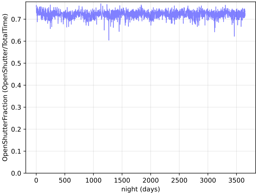
too_ignore_100_1v3.4_10yrs Per night: OpenShutterFraction
