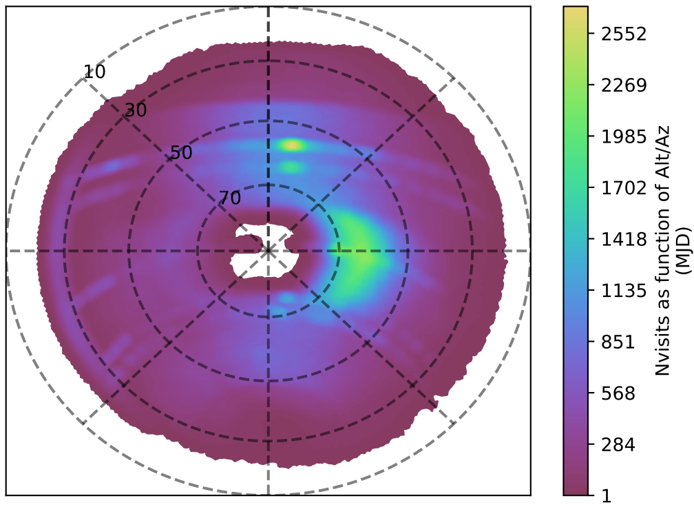
too_ignore_100_1v3.4_10yrs r band: Nvisits as function of Alt/Az
