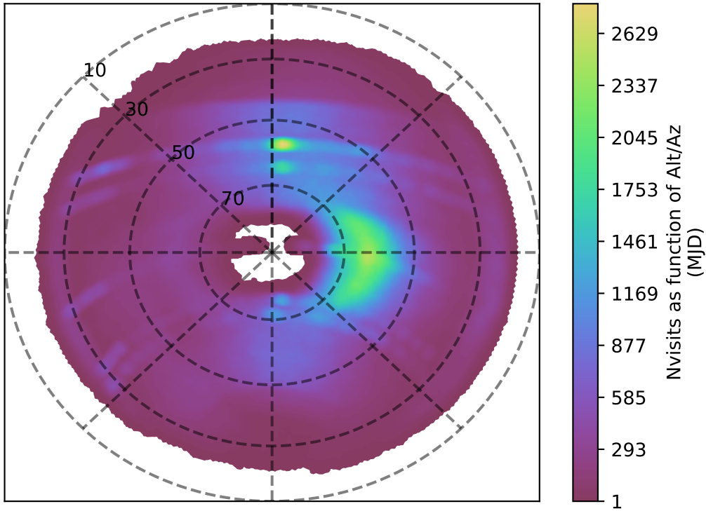
too_ignore_100_1v3.4_10yrs i band: Nvisits as function of Alt/Az
