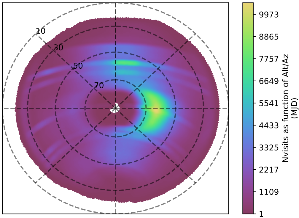
too_ignore_100_1v3.4_10yrs all bands: Nvisits as function of Alt/Az
