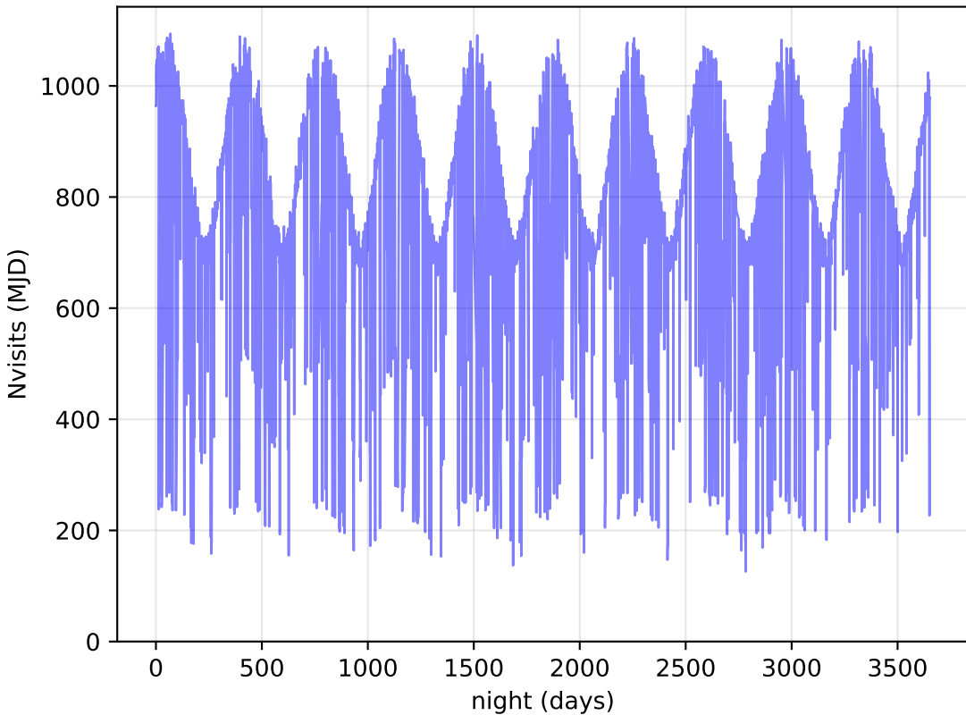
too_ignore_100_1v3.4_10yrs All visits: Nvisits
