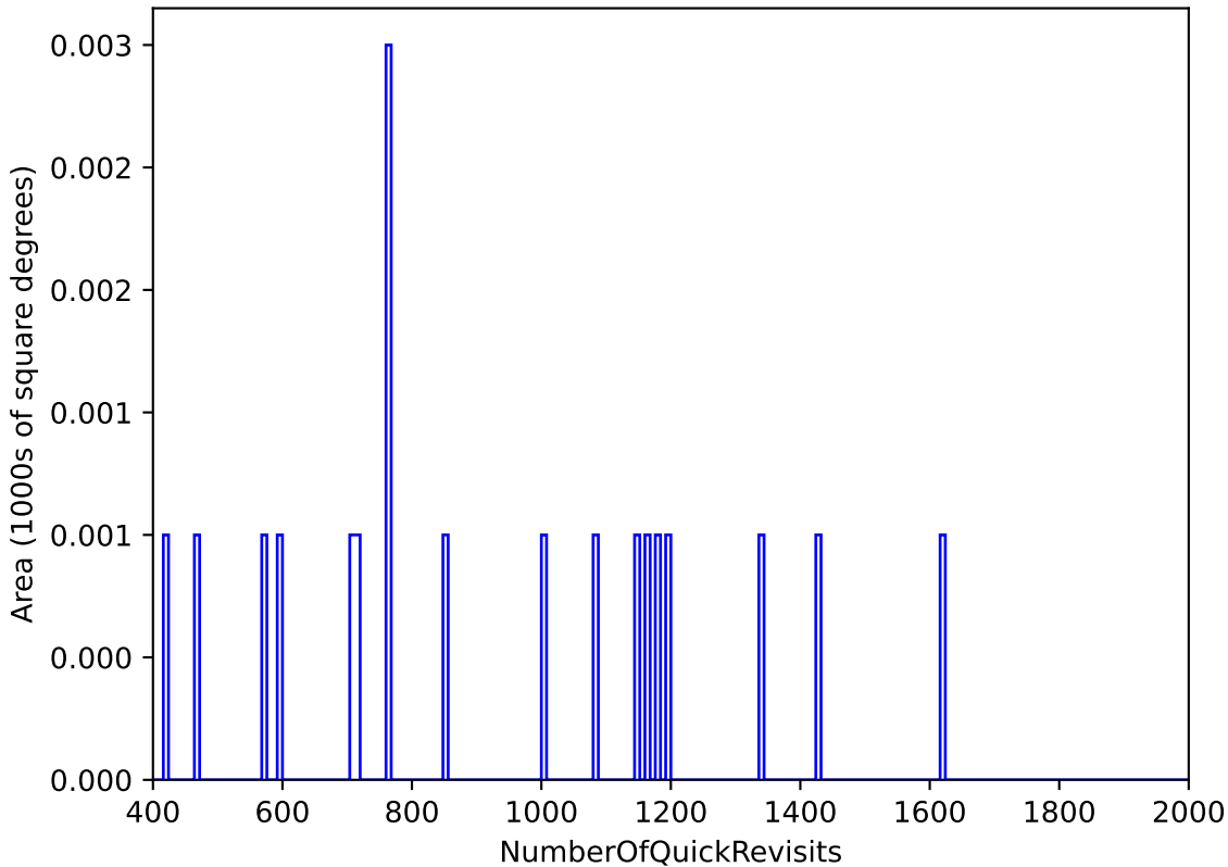
too_ignore_100_1v3.4_10yrs WFD: NumberOfQuickRevisits
