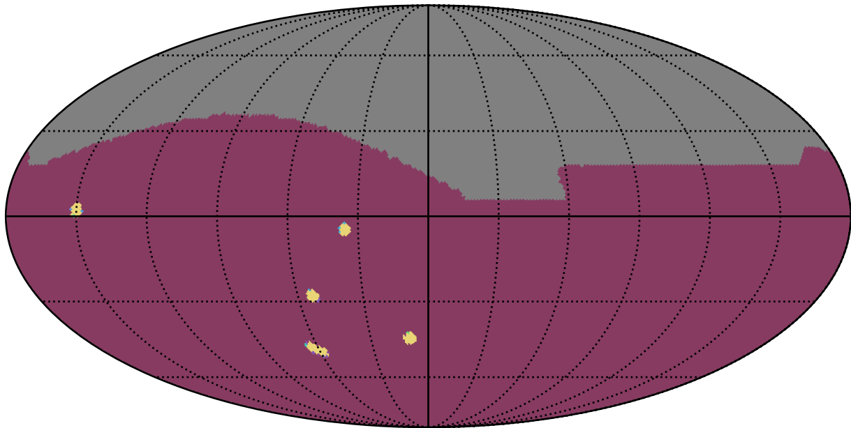
too_ignore_100_1v3.4_10yrs All sky: NumberOfQuickRevisits
