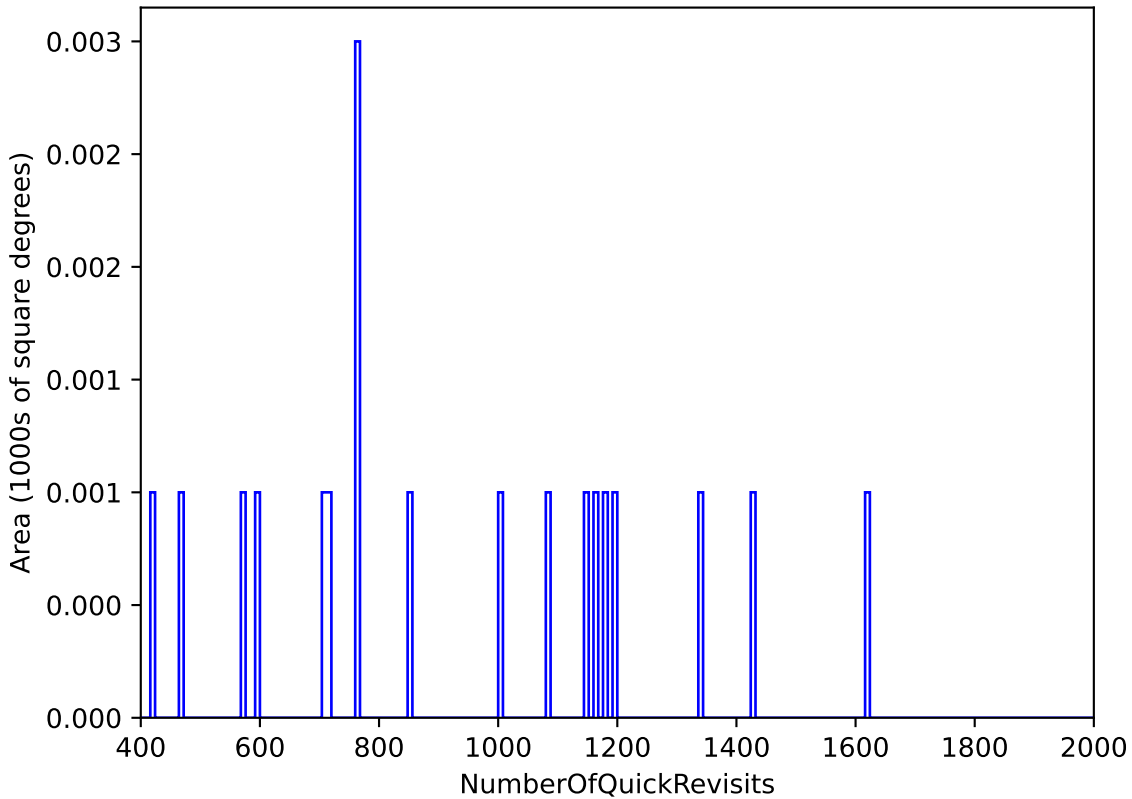
too_ignore_100_1v3.4_10yrs All sky: NumberOfQuickRevisits
