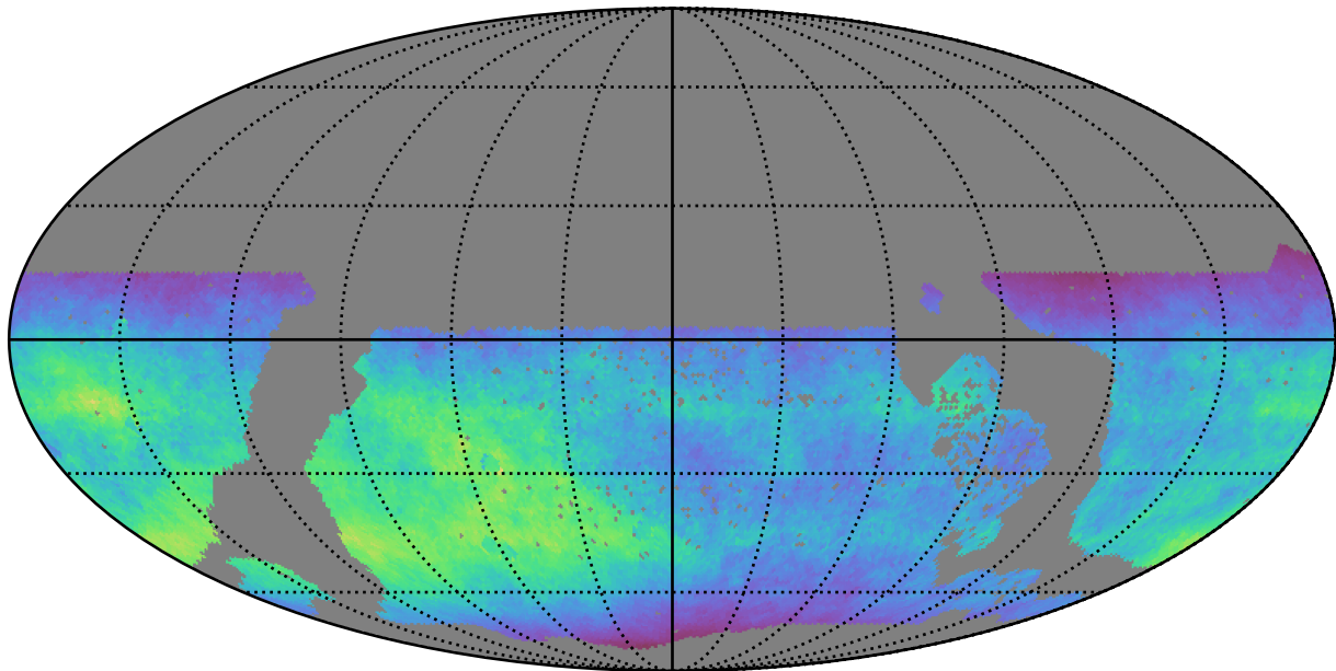
too_ignore_100_1v3.4_10yrs WFD z band: Normalized Teff
