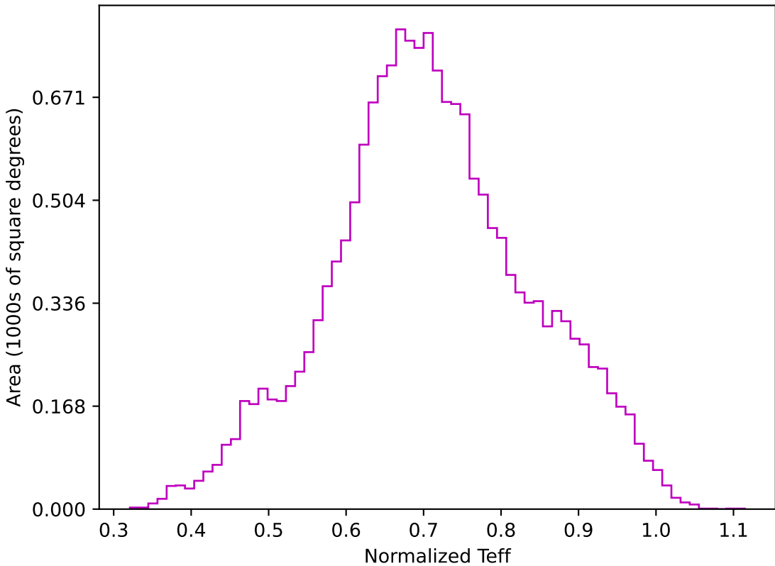
too_ignore_100_1v3.4_10yrs WFD z band: Normalized Teff
