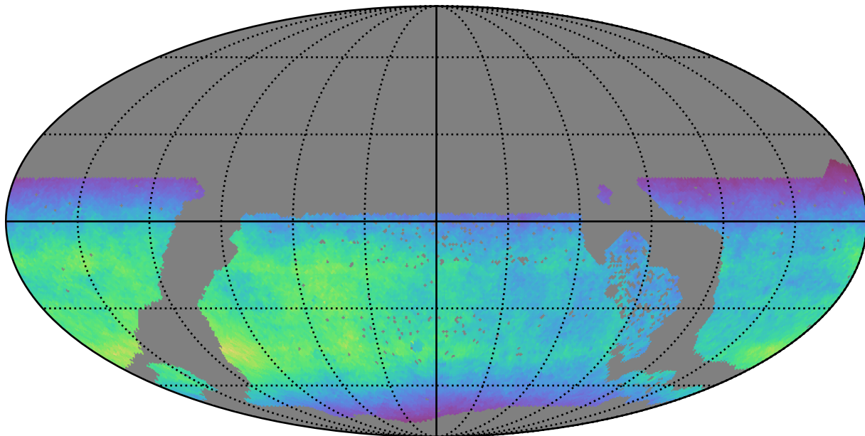
too_ignore_100_1v3.4_10yrs WFD y band: Normalized Teff
