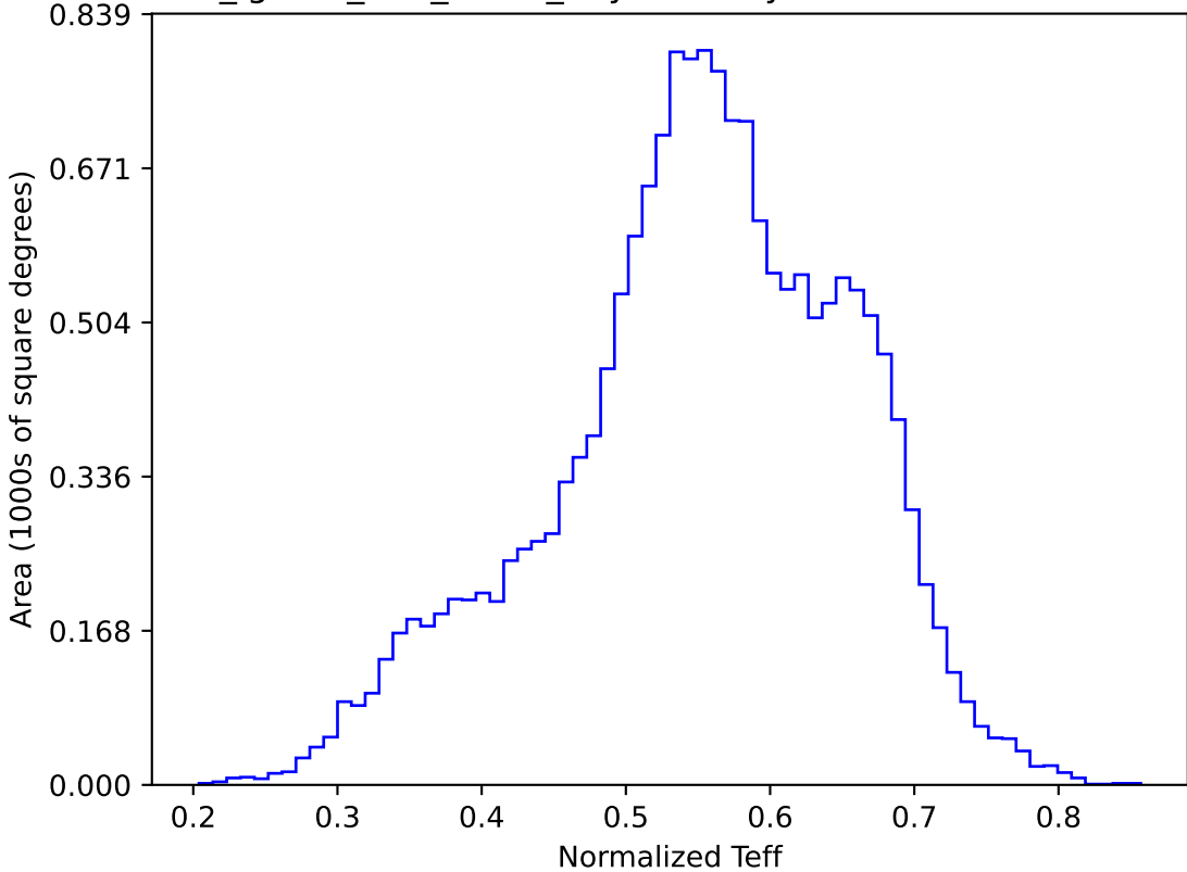
too_ignore_100_1v3.4_10yrs WFD y band: Normalized Teff
