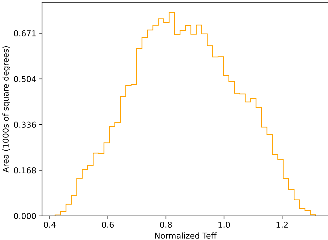
too_ignore_100_1v3.4_10yrs WFD r band: Normalized Teff
