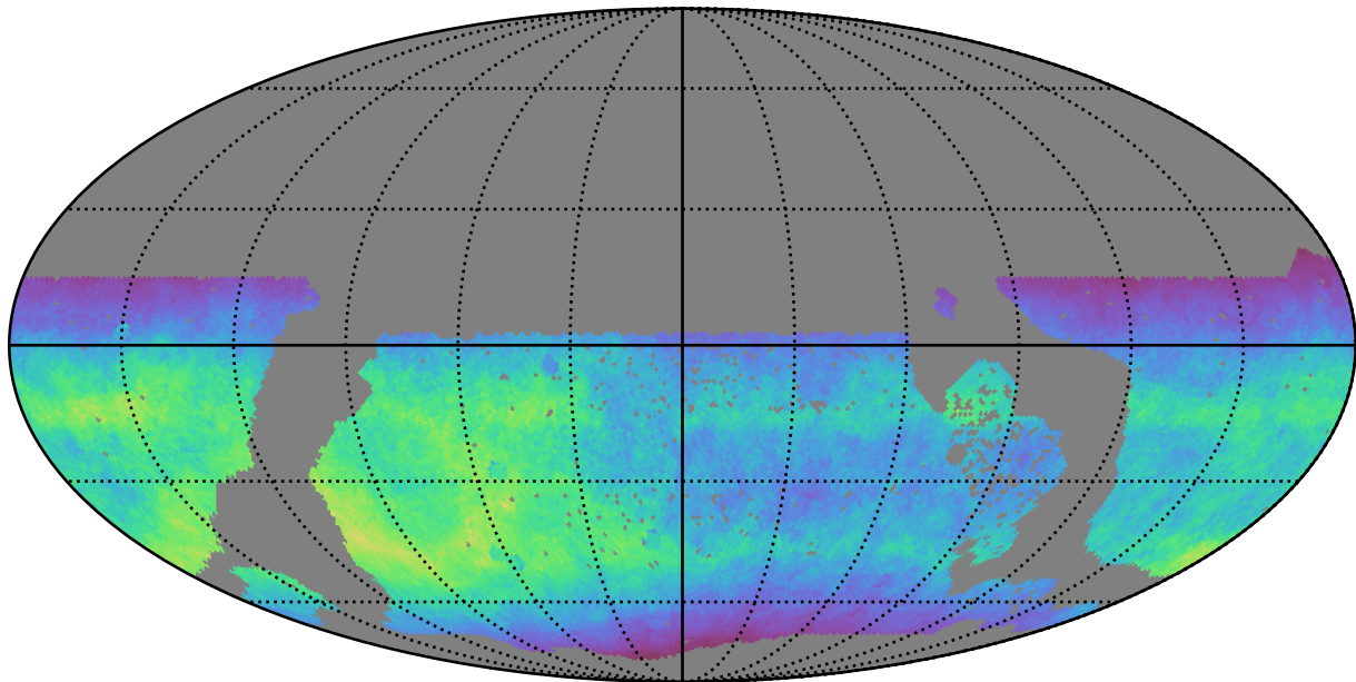
too_ignore_100_1v3.4_10yrs WFD i band: Normalized Teff
