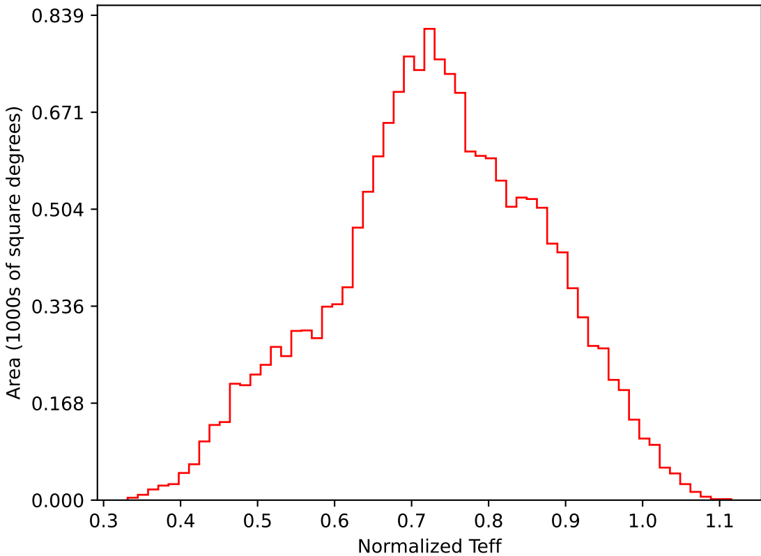
too_ignore_100_1v3.4_10yrs WFD i band: Normalized Teff
