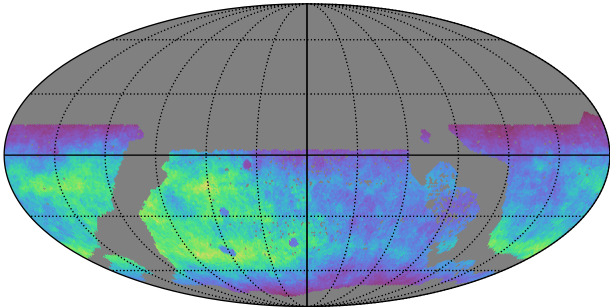
too_ignore_100_1v3.4_10yrs WFD g band: Normalized Teff
