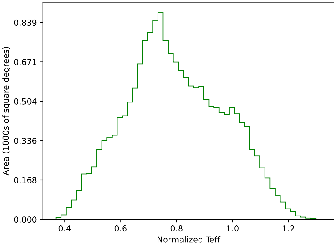
too_ignore_100_1v3.4_10yrs WFD g band: Normalized Teff
