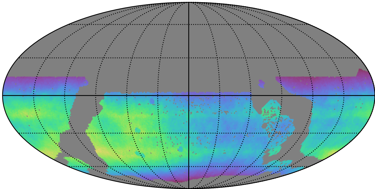
too_ignore_100_1v3.4_10yrs WFD all bands: Normalized Teff
