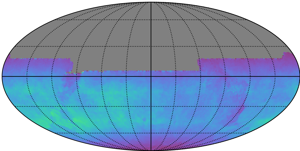
too_ignore_100_1v3.4_10yrs All sky y band: Normalized Teff
