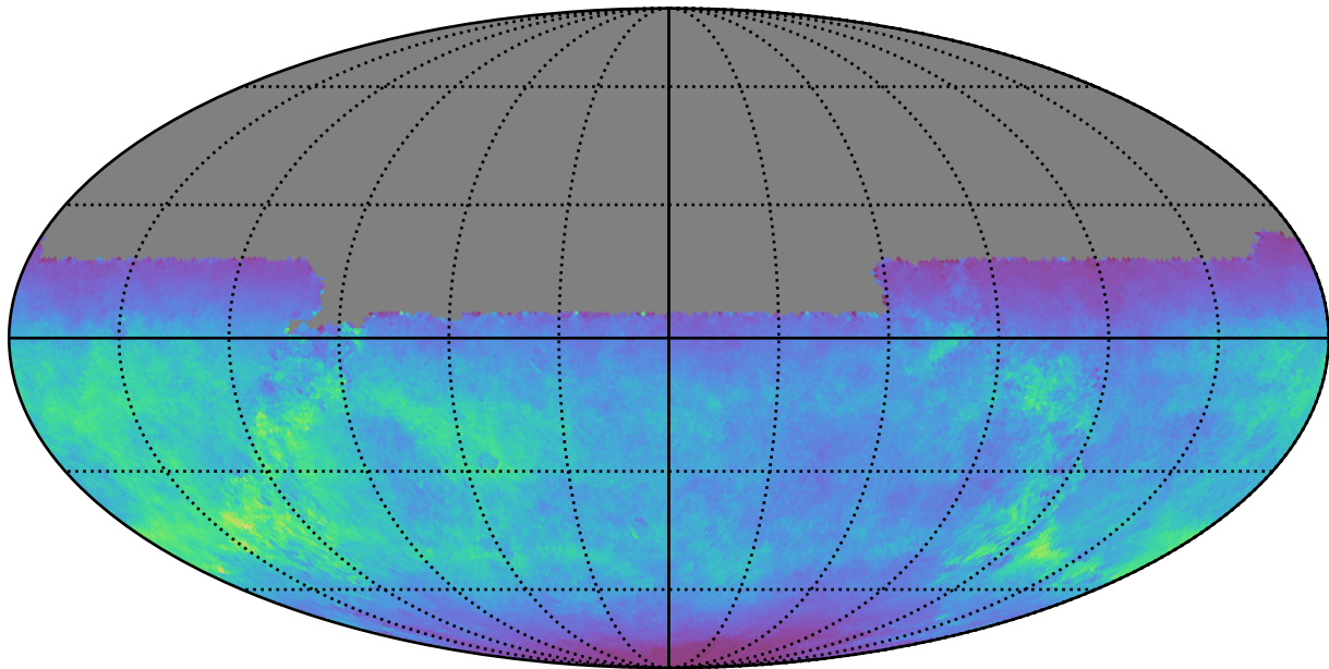
too_ignore_100_1v3.4_10yrs All sky u band: Normalized Teff
