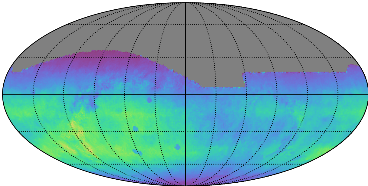
too_ignore_100_1v3.4_10yrs All sky r band: Normalized Teff
