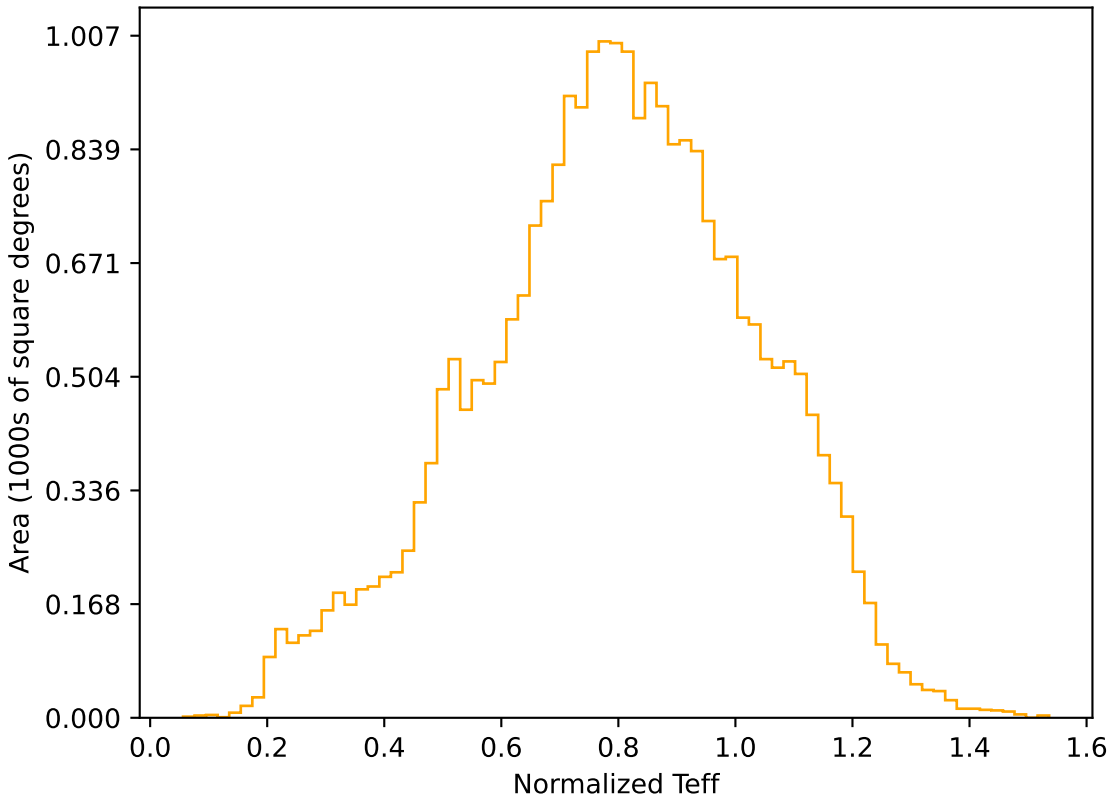
too_ignore_100_1v3.4_10yrs All sky r band: Normalized Teff
