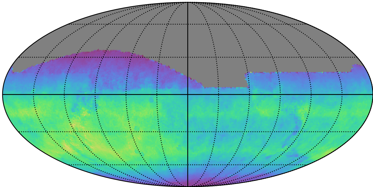
too_ignore_100_1v3.4_10yrs All sky i band: Normalized Teff
