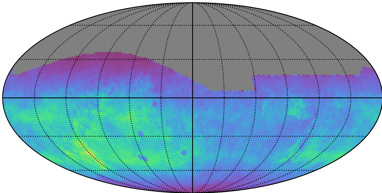
too_ignore_100_1v3.4_10yrs All sky g band: Normalized Teff
