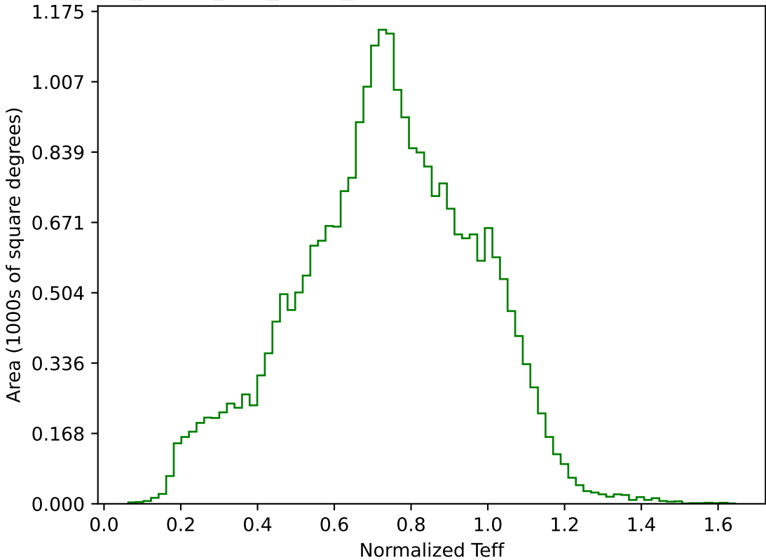
too_ignore_100_1v3.4_10yrs All sky g band: Normalized Teff
