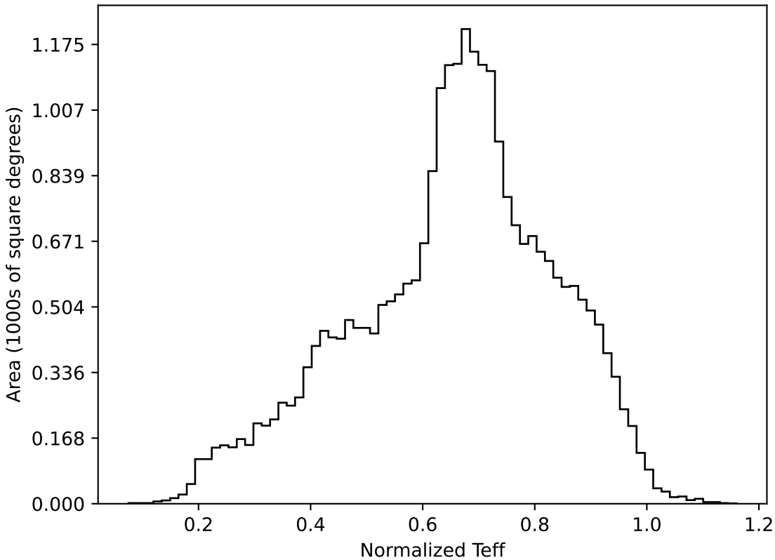
too_ignore_100_1v3.4_10yrs All sky all bands: Normalized Teff
