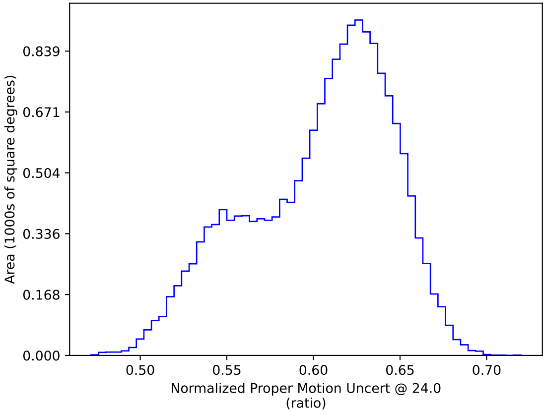
too_ignore_100_1v3.4_10yrs WFD: Normalized Proper Motion Uncert @ 24.0
