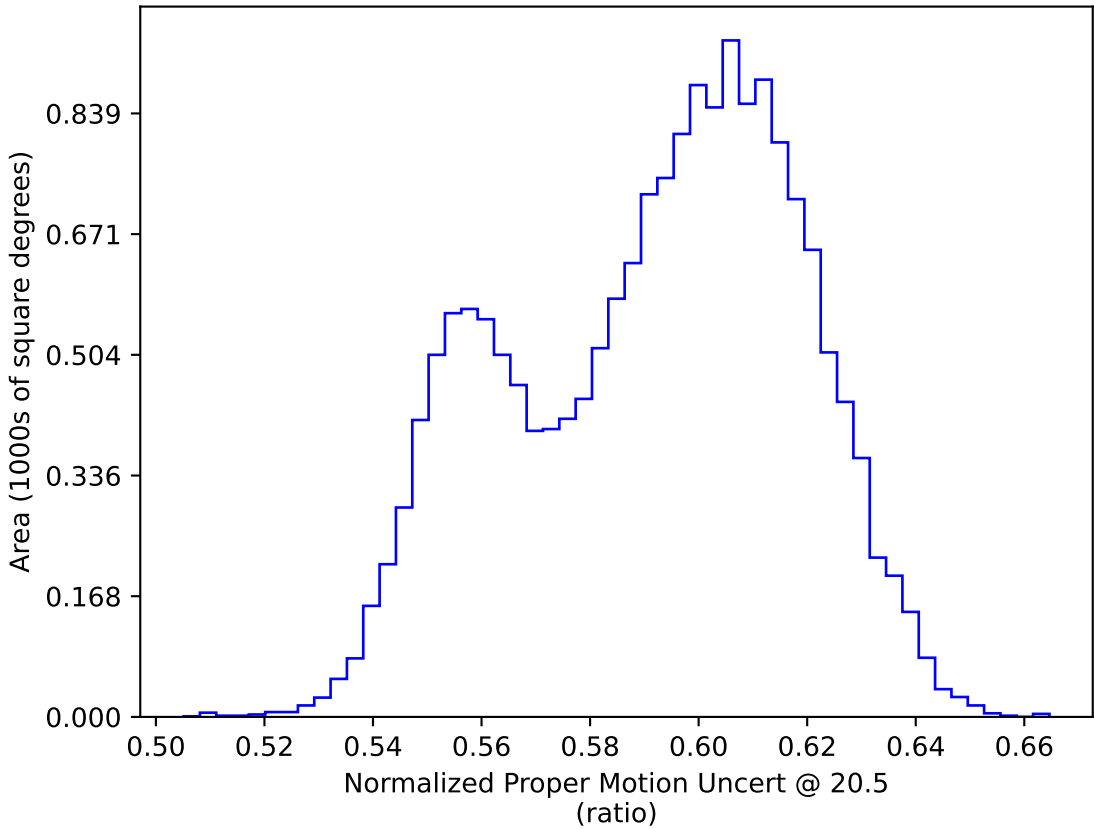
too_ignore_100_1v3.4_10yrs WFD: Normalized Proper Motion Uncert @ 20.5
