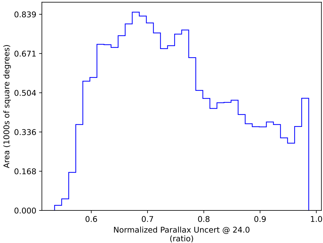
too_ignore_100_1v3.4_10yrs WFD: Normalized Parallax Uncert @ 24.0
