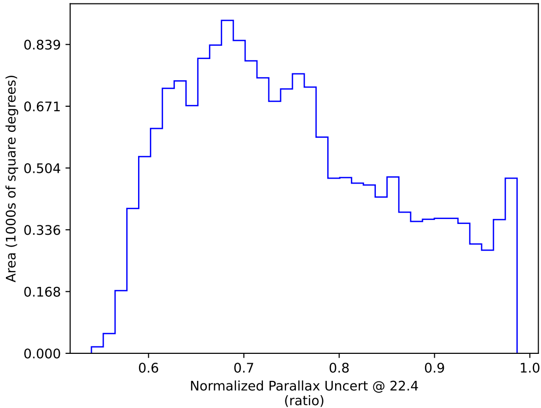
too_ignore_100_1v3.4_10yrs WFD: Normalized Parallax Uncert @ 22.4
