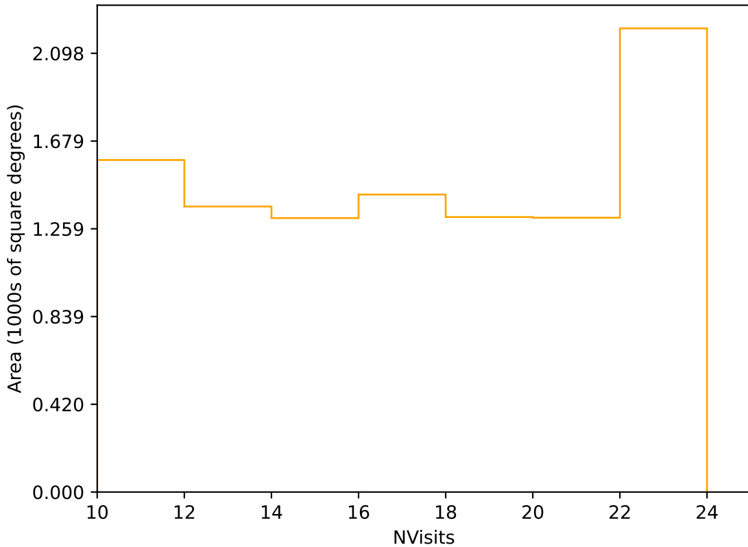
too_ignore_100_1v3.4_10yrs Yr 3-4 r band: NVisits
