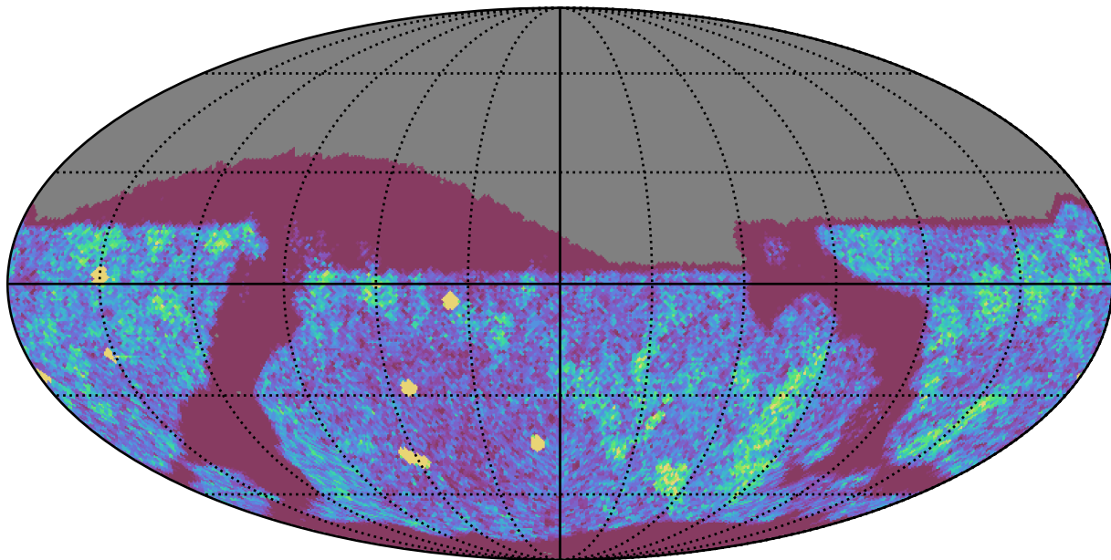
too_ignore_100_1v3.4_10yrs Yr 1 z band: NVisits
