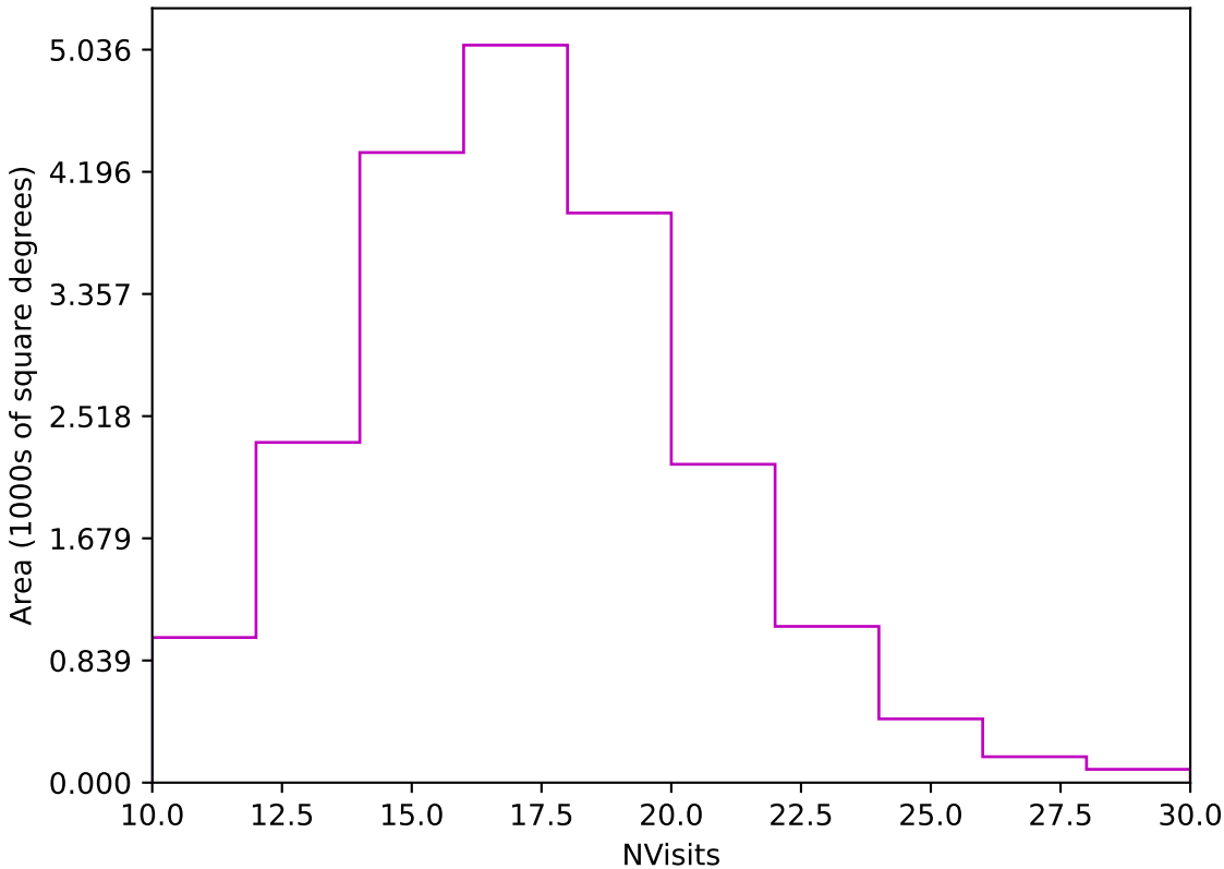
too_ignore_100_1v3.4_10yrs Yr 1 z band: NVisits
