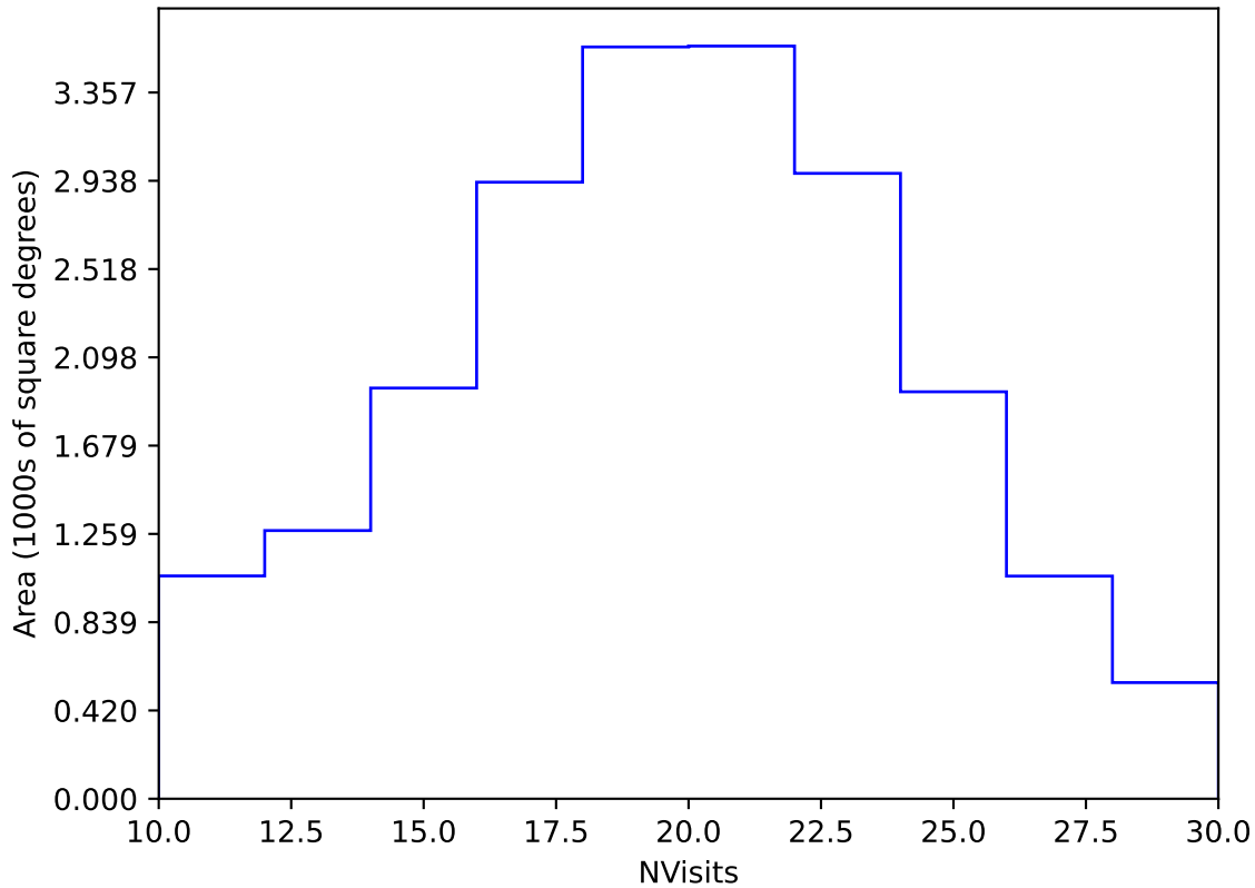
too_ignore_100_1v3.4_10yrs Yr 1 y band: NVisits
