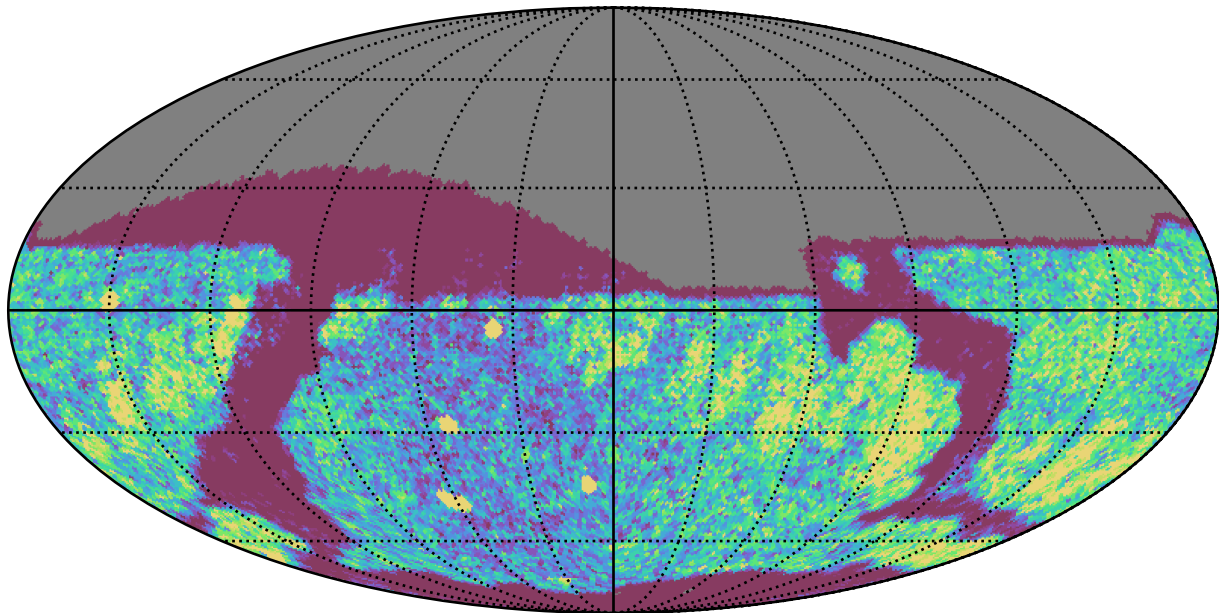
too_ignore_100_1v3.4_10yrs Yr 1 r band: NVisits
