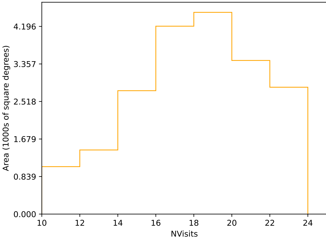
too_ignore_100_1v3.4_10yrs Yr 1 r band: NVisits
