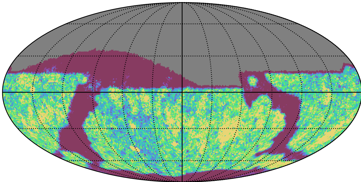
too_ignore_100_1v3.4_10yrs Yr 1 i band: NVisits
