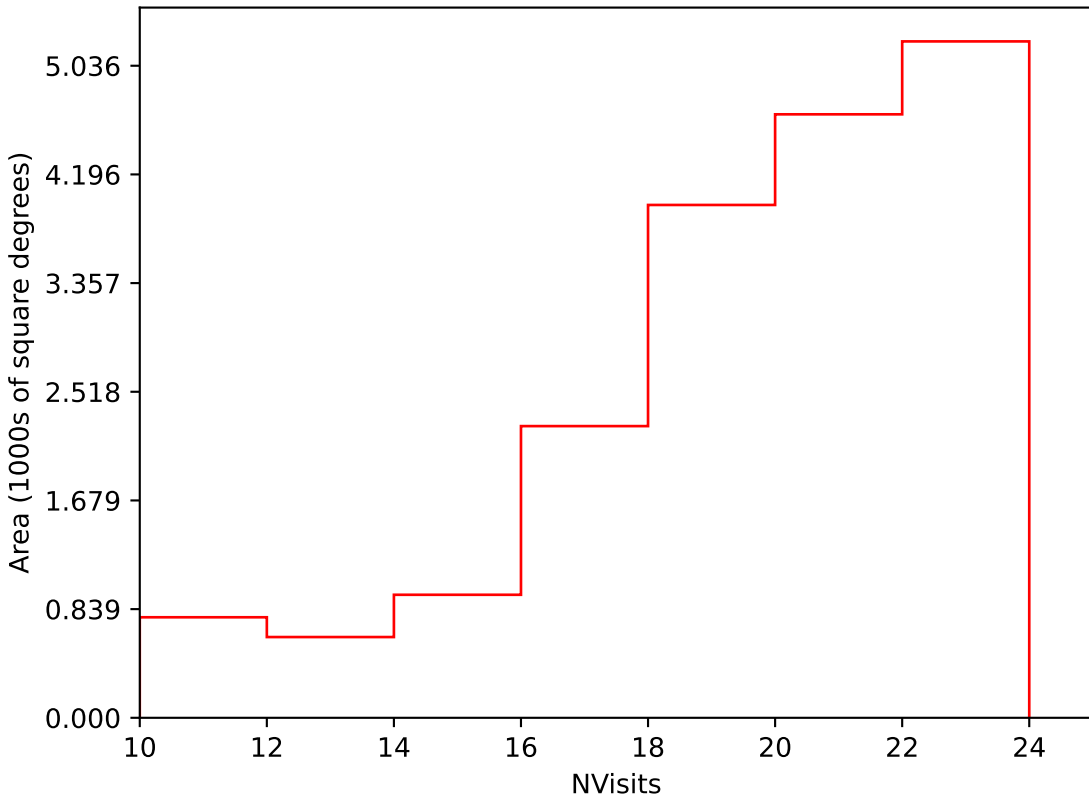
too_ignore_100_1v3.4_10yrs Yr 1 i band: NVisits
