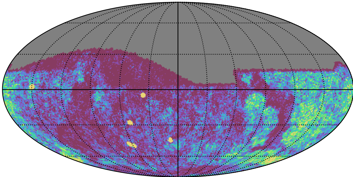
too_ignore_100_1v3.4_10yrs Yr 1 g band: NVisits
