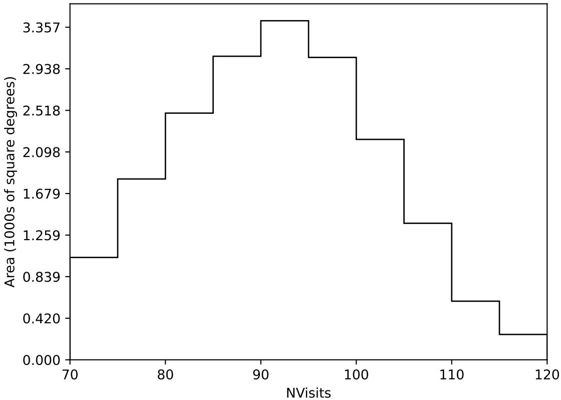
too_ignore_100_1v3.4_10yrs Yr 1 all bands: NVisits
