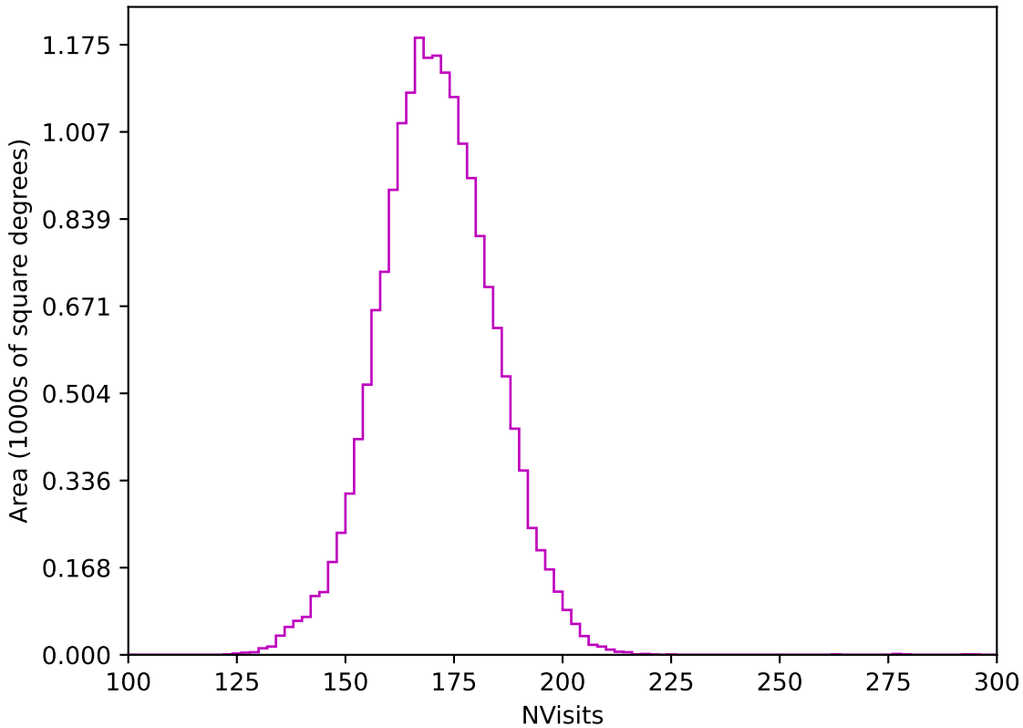
too_ignore_100_1v3.4_10yrs WFD z band: NVisits
