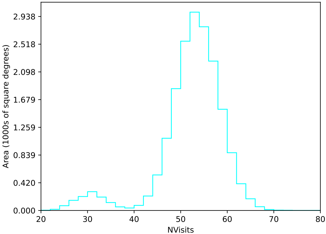
too_ignore_100_1v3.4_10yrs WFD u band: NVisits
