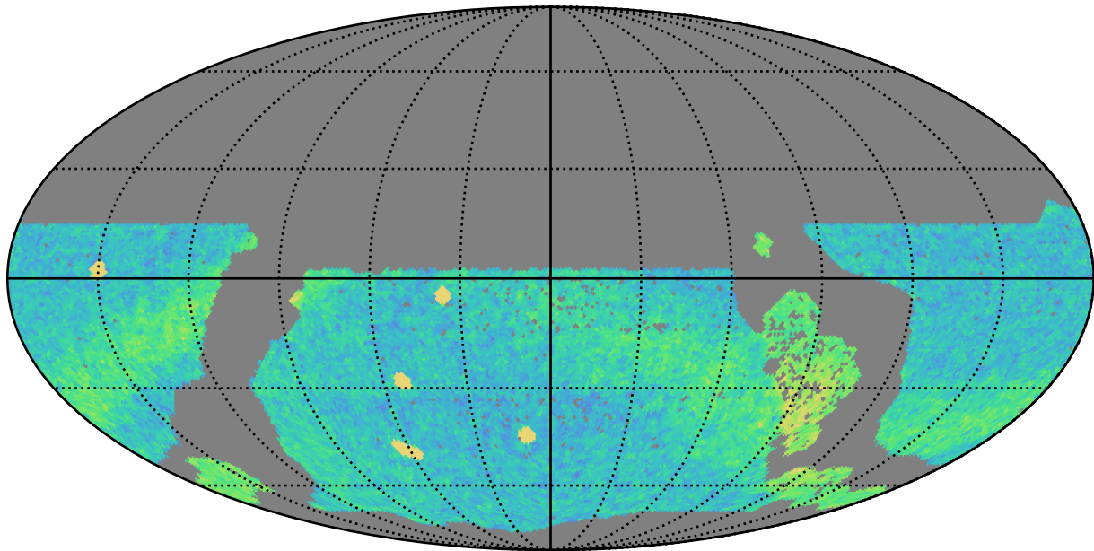
too_ignore_100_1v3.4_10yrs WFD r band: NVisits
