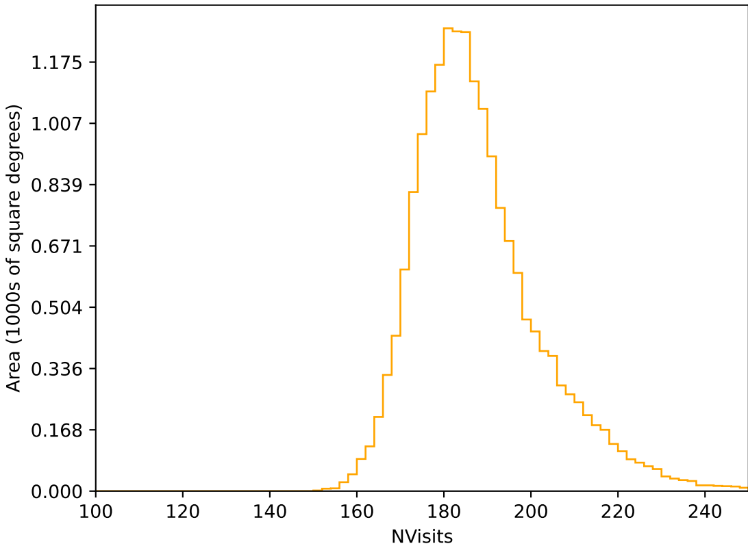
too_ignore_100_1v3.4_10yrs WFD r band: NVisits
