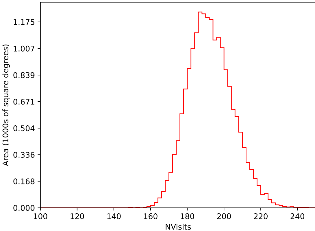
too_ignore_100_1v3.4_10yrs WFD i band: NVisits
