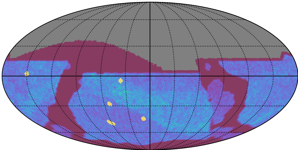
too_ignore_100_1v3.4_10yrs All sky z band: NVisits
