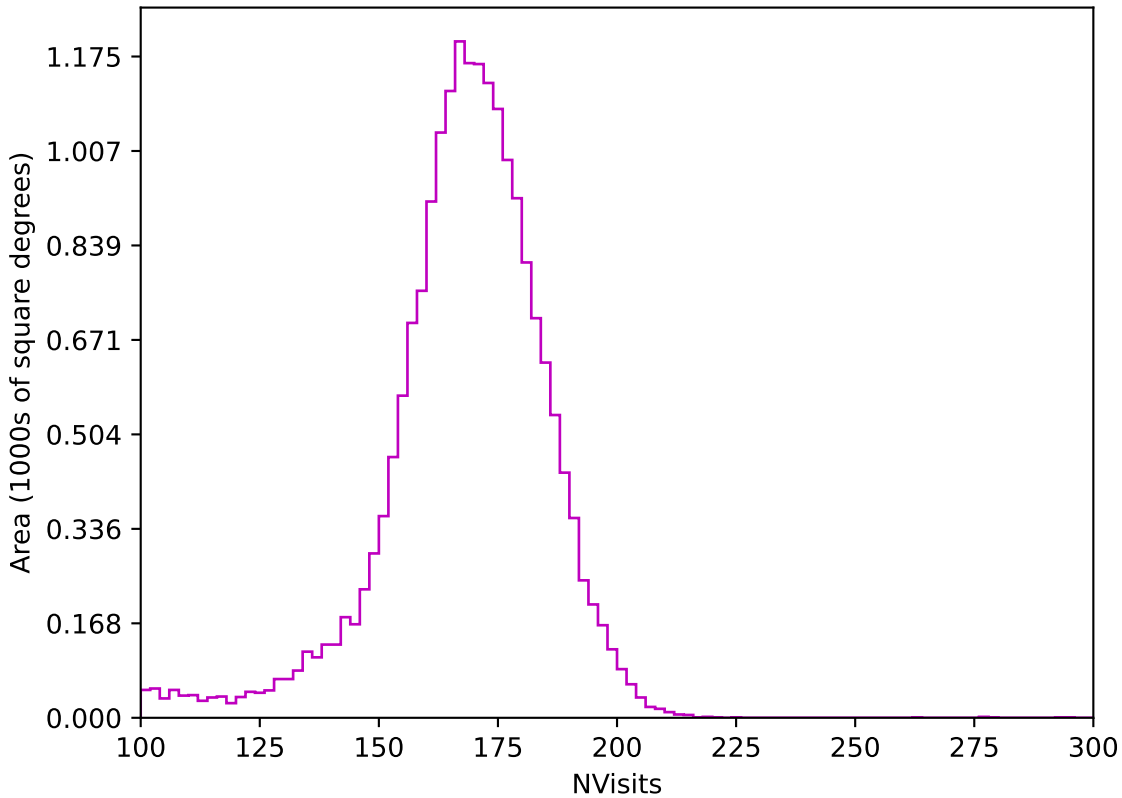
too_ignore_100_1v3.4_10yrs All sky z band: NVisits
