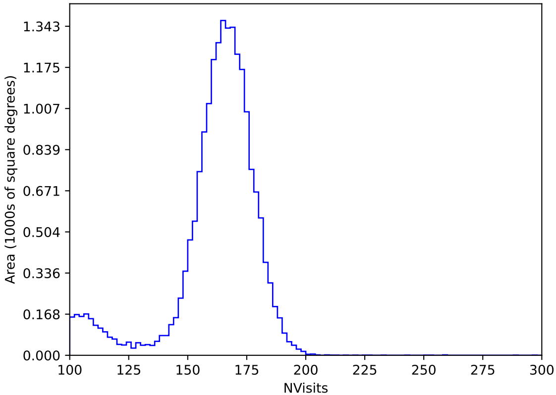
too_ignore_100_1v3.4_10yrs All sky y band: NVisits
