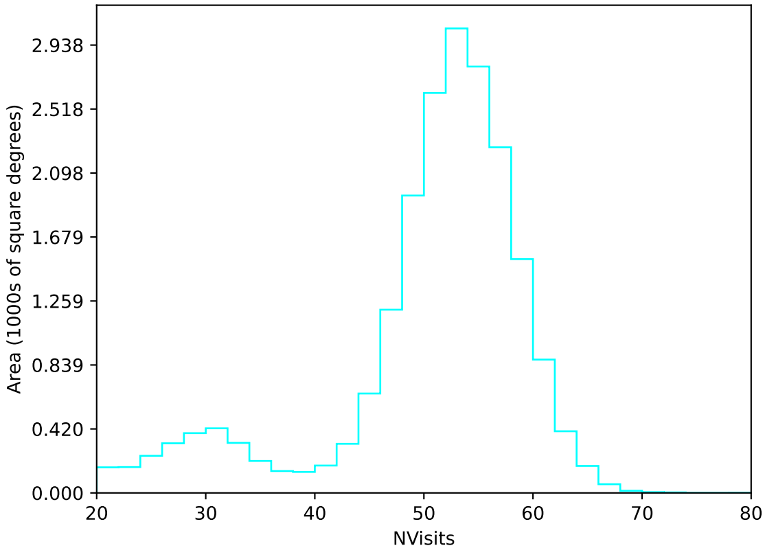
too_ignore_100_1v3.4_10yrs All sky u band: NVisits
